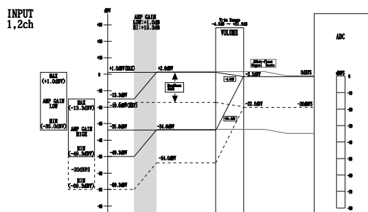
Portacapture X8 LEVEL DIAGRAM
